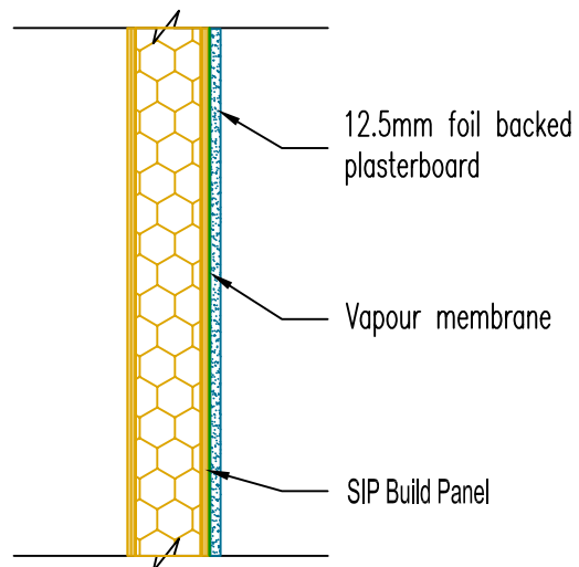
PLASTERBOARD FIXED OVER VAPOR MEMBRANE OVER PANEL
