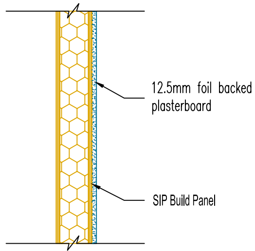
PLASTERBOARD FIXED DIRECTLY TO PANEL
