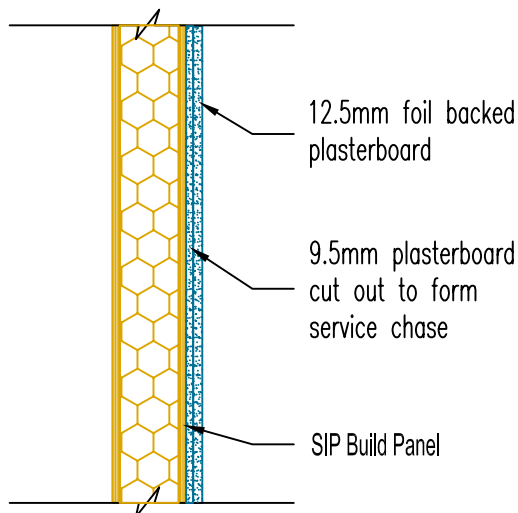
DOUBLE LAYER OF PLASTERBOARD FIXED DIRECTLY TO PANEL
