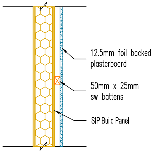
PLASTERBOARD FIXED USING SW BATTENS
